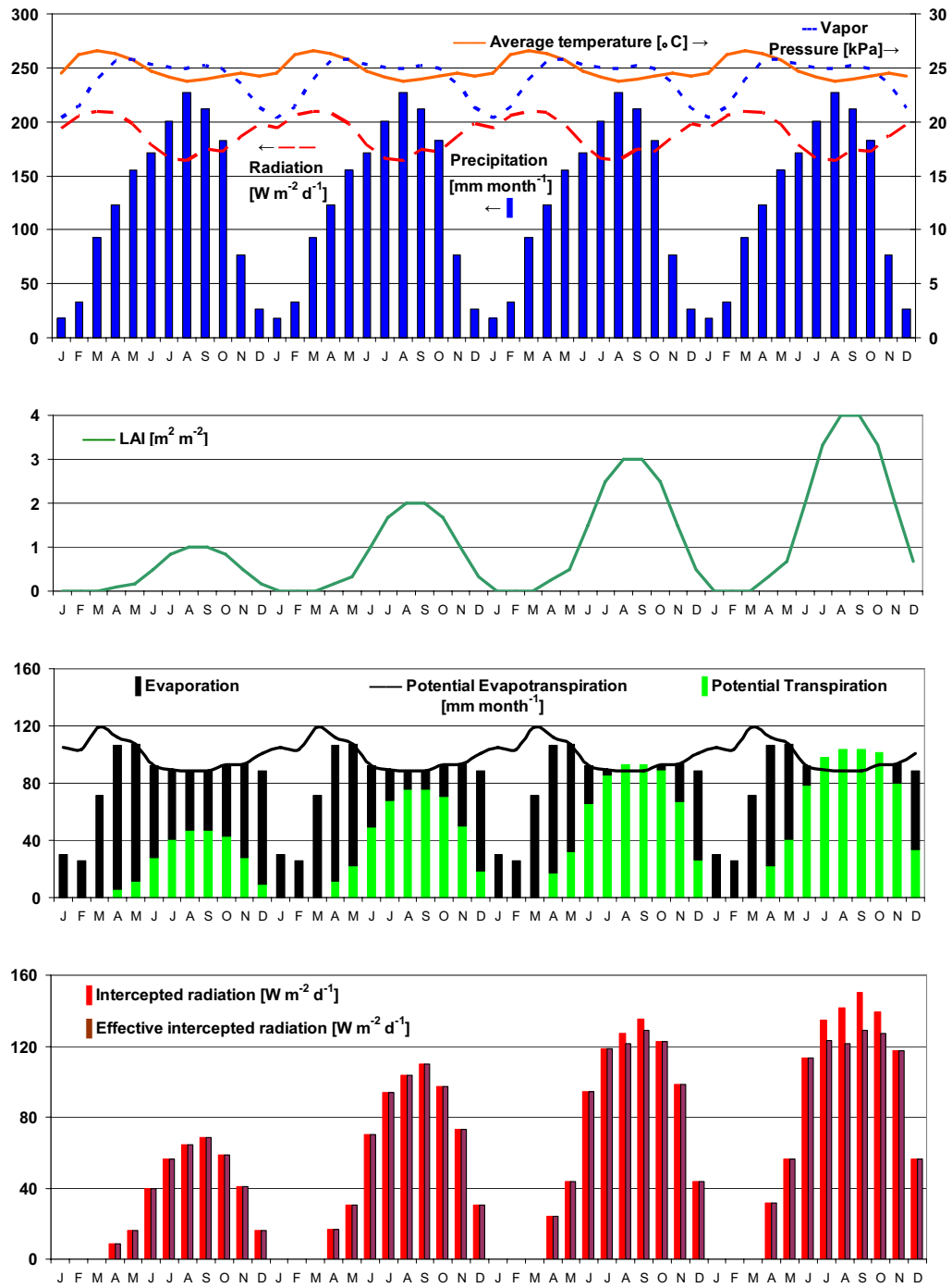
Figure 8. 4 years average climate data for Bangui, Central African Republic ( 4^{\circ} 14' N , 18^{\circ} 21' E ) and the development of a virtual J. curcas canopy (LAI), with effects on evapotranspiration and (effective) intercepted radiation.
